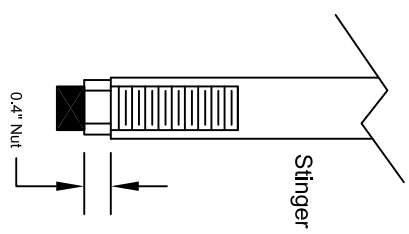
Reverse Mount Proximity Probe 5.5mm (0.22") Probe Tip
