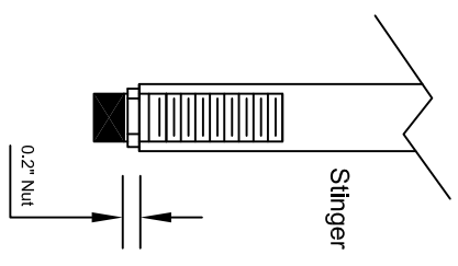
3/8"-24 Proximity Probe 7mm (0.28") Probe Tip
